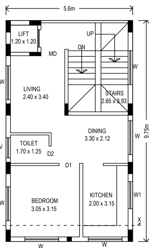
TYPICAL FIRST & SECOND FLOOR PLAN
